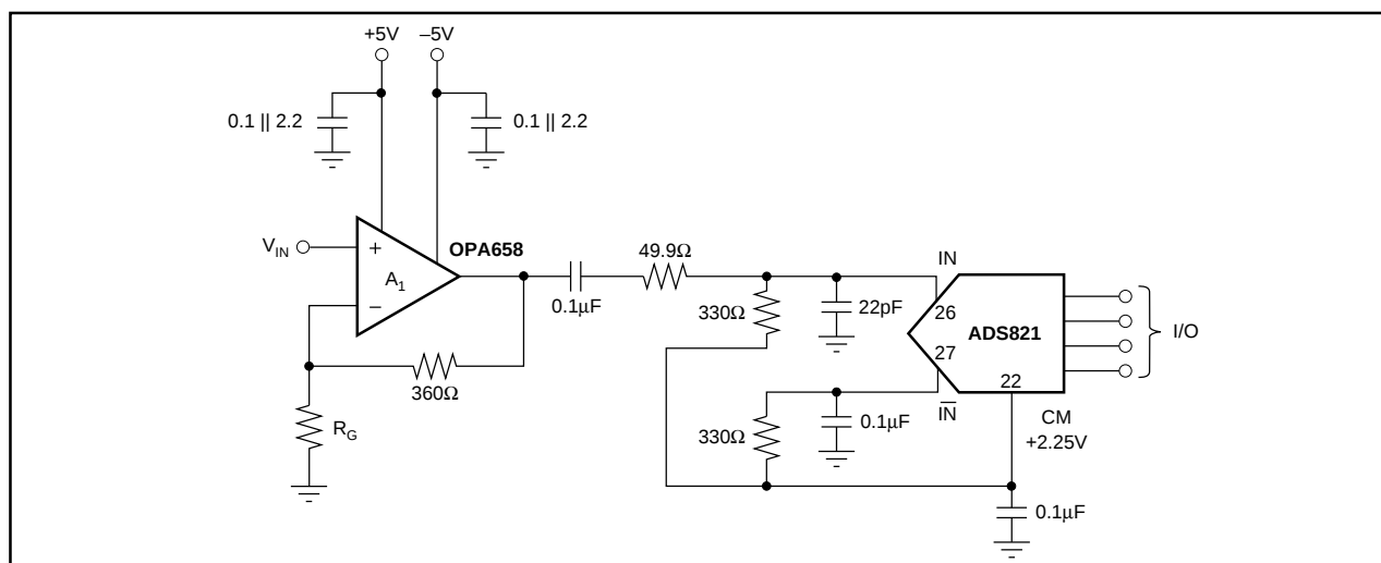
FIGURE 6. Low-Cost AC-Coupled Single-Ended Input Circuit.
